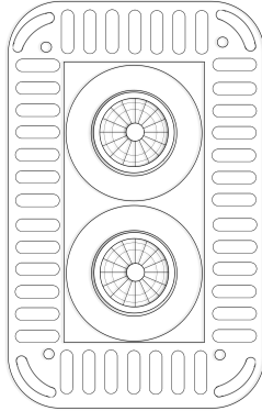
Cut Out: 92x184mm Outer Dimensions: 75x150mm
