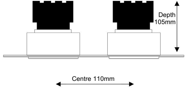
Cut Out: Ø2x95mm Visible Diameter: Ø2x75mm
