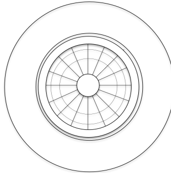
Cut Out: Ø64mm Outer Diameter: Ø75mm
